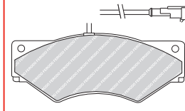
FVR1405 BRE 29123 107 x 61 x 20mm
