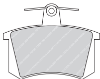
FDB1407 ATE 23762 155 x 72.8 x 19.3mm
