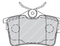
FDB4250 TRW 24765 87.2 x 53 x 16.6mm
