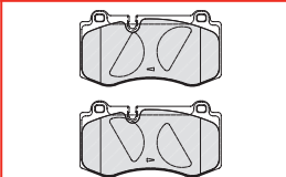
FDB4055 BRE 23960 141.6 x 76.2 x 17.6mm
