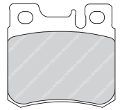
FDB1037 ATE 21153 100 x 74 x 16mm
