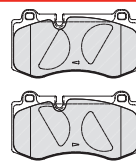
FDB4055 BRE 23960 141.6 x 76.2 x 17.6mm
