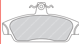
FVR239 PER 29784 149 x 74 x 18mm
