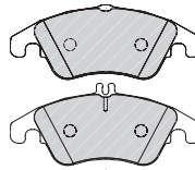
FDB1979 TRW 24456 188 x 80 x 19.2mm
