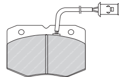
FVR1315 BRE 29121 165 x 66 x 18mm
