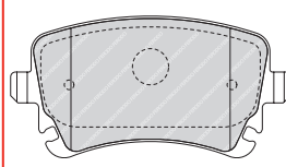
FDB1832 ATE 23885 193 x 72.6 x 19.9mm
