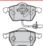
FDB1717 ATE 20676 156 x 74 x 20.1mm
