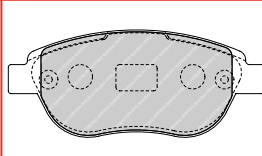
FDB1476 BOS 23600 137 x 57.4 x 19.3mm
