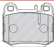
FDB4346 ATE 24177 193.1 x 81.9 x 20.8mm
