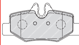
FVR1494 BOS 24008 99 x 48.8 x 18.5mm
