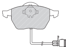
FDB1629 ATE 23762 155/156 x 72.8 x 20.2mm
