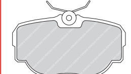
FDB4104 TRW 25021 192.6 x 72.1 x 18.6mm
