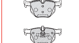
FDB4287 ATE 24436 193.1/192.4 x 96.6 x 19.8/20.3mm
