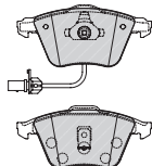
FDB1709 TRW 23280 63.5/77.2 x 75.6/74.7 x 18mm
