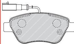
FDB1466 BOS 23705 123 x 53.4 x 17.1mm
