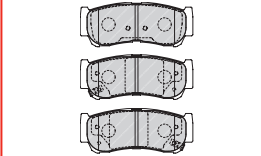
FDB1910 MAN 24488 118.6 x 47 x 15.4/15.9mm
