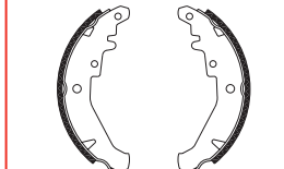
FSB4077 BOS 185 x 29mm
