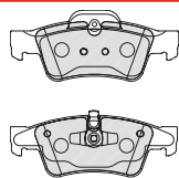
FDB1831 ATE 23923 140.2/141.4 x 51.8/59.6 x 17.6mm
