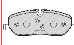
FDB1615 TRW 24191 162.6 x 58 x 18mm
