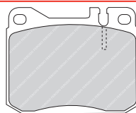
FDB799 ATE 21305 62 x 69 x 16mm
