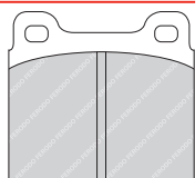
FDB646 ATE 21153 100 x 74 x 17.5mm
