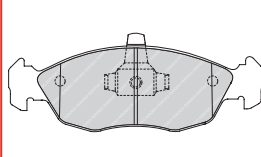
FDB1477 LUC 23346 130 x 56 x 19mm
