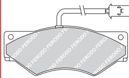
FVR1352 BRE 29139 110 x 73 x 18.3mm
