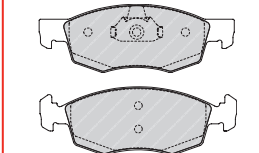
FDB1376 ATE 23552 150 x 52.5 x 17.8mm
