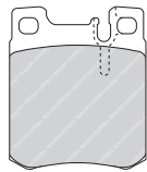
FDB1322 ATE 21898 64 x 78 x 15.5mm
