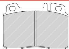
FDB1594 ATE 23723 156/155 x 66.9/62.5 x 17.5mm
