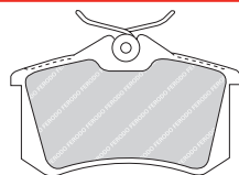
FDB1788 TRW 20961 87 x 53 x 17mm
