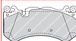
FDB4373 BRE 24681 189.7 x 93.2 x 17.6mm
