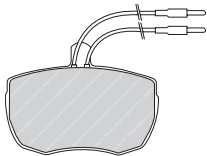
FVR1351 WAB 29138 149 x 69 x 18mm
