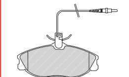
FDB1168 ATE 21430 142 x 47.5 x 17mm
