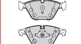
FDB4382 ATE 24688 155.2 x 68.3 x 19/20.0mm
