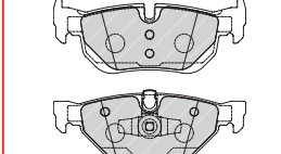
FDB4286 ATE 23731 139.7 x 67.8 x 16.7mm
