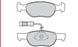
FDB1349 LUC 23517 96 x 43.9 x 16.6mm
