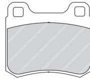
FDB979 ATE 20687 62 x 55 x 15.5mm
