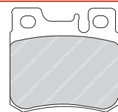
FDB1526 ATE 23334 141 x 59.5 x 15.8mm
