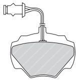
FDB872 LKD 23471 89 x 69 x 15mm
