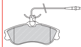
FDB4250 TRW 24765 87.2 x 53 x 16.6mm
