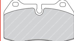
FDB4221 ATE 24161 155.4 x 68.5 x 19.8mm
