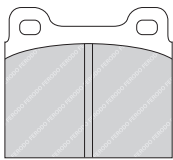
FDB644 ATE 21197 62 x 59 x 15.5mm
