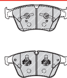
FDB4346 ATE 24177 193.1 x 81.9 x 20.8mm
