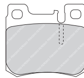
FDB1322 ATE 21898 64 x 78 x 15.5mm
