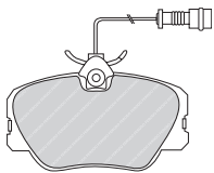
FDB1401 KEL 23189 140 x 50 x 16.5mm
