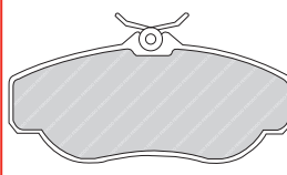
FDB980 LUC 23452 145 x 67 x 18.2mm
