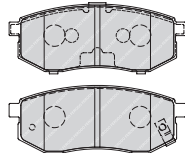
FDB1970 SUM 23608 103 x 39.4 x 15.5mm
