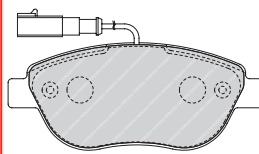
FDB1467 BOS 23708 137 x 57.3 x 18.4mm
