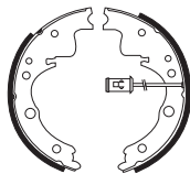
FSB407 LKD 254 x 89mm
