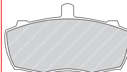
FVR836 LKD 20904 127 x 71 x 18mm
