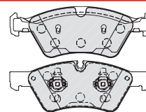
FDB1830 ATE 23922 193.3/194.5 x 70.1 x 21mm
