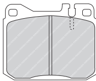
FDB693 ATE 21301 62 x 54 x 15.5mm
