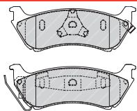
FDB1831 ATE 23923 140.2/141.4 x 51.8/59.6 x 17.6mm
