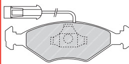
FDB1299 ATE 21637 156/155 x 58/63 x 18.5mm
