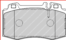
FDB4189 ATE 24151 193.1 x 80.3 x 20.9/20.3mm
