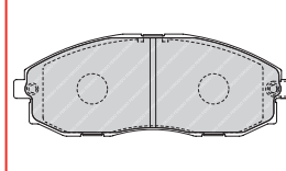
FVR1498 MAN 23536 147 x 53.8 x 16.5mm
