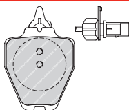
FDB1709 TRW 23280 63.5/77.2 x 75.6/74.7 x 18mm
