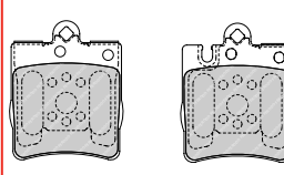
FDB1979 TRW 24456 188 x 80 x 19.2mm
