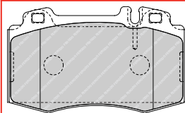
FDB1810 BRE 23541 97.6 x 78.5 x 17.2mm
