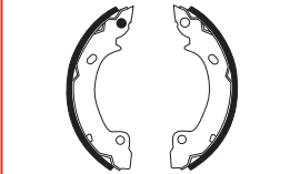
FSB4084 MAN 254 x 57mm
