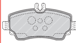
FVR1044 ATE 21278 64 x 57.4 x 17mm
