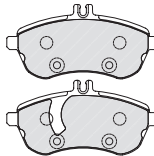
FDB1978 LUC 24306 146.2 x 71.5 x 20.6mm
