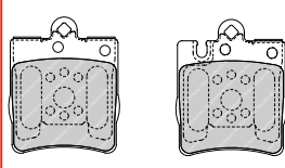
FDB1907 BRE 23945 101.7 x 79.5 x 16.5mm
