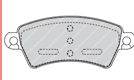
FDB1370 BOS 23396 131 x 51.2 x 18mm
