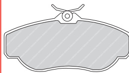
FDB1996 BRE 20217 131.8 x 77.3 x 17.3mm
