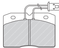
FVR709 WAB 20465 149 x 69 x 18mm
