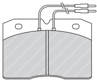
FVR655 BRE 29041 110 x 73 x 18.3mm
