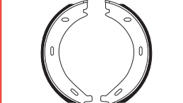
FSB536 LUC 180 x 20mm
