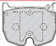
FDB1810 BRE 23541 97.6 x 78.5 x 17.2mm
