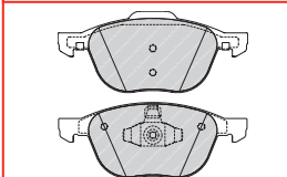
FDB4412 ATE - 138.6 x 73.9 x 16.7mm
