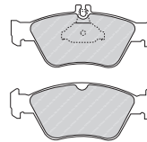
FDB1429 TRW 23144 132 x 69.8/62.05 x 19.5mm
