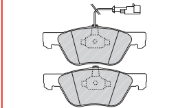
FDB1376 ATE 23552 150 x 52.5 x 17.8mm
