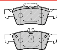
FDB4055 BRE 23960 141.6 x 76.2 x 17.6mm
