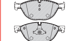
FDB4285 ATE 25045 192.3/193 x 79.5 x 18.2/20mm
