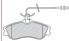
FDB1399 BOS 23599 137 x 50.8 x 19mm
