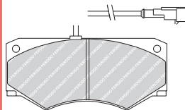
FVR1351 WAB 29138 149 x 69 x 18mm
