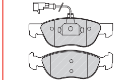
FDB1377 ATE 20907 150 x 52.5 x 17.8mm
